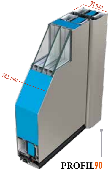
PROFIL 90 Curved Frame Telaio Curved / Dormant Arrondi
